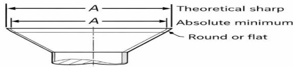
Enlarged View of Head
