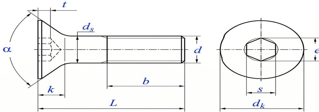
Dimensions of Flat Countersunk Head Cap Screws
